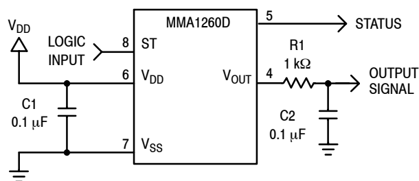
Pin No. Pin Name Description 1 thru 3 V_{SS} Redundant connections to the internal V_{SS} and may be left unconnected. 4 V_{OUT} Output voltage of the accelerometer. 5 STATUS Logic output pin used to indicate fault. 6 V_{DD} The power supply input. 7 V_{SS} The power supply ground. 8 ST Logic input pin used to initiate self-test. 9 thru 13 Trim pins Used for factory trim. Leave unconnected. 14 thru 16 — No internal connection. Leave unconnected.
